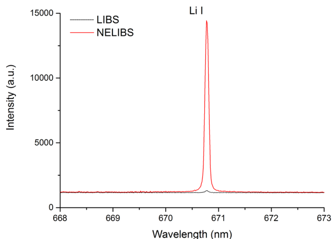
Figure 10. Comparison between the NELIBS and LIBS signal of Li in 1 \mu\text{L} of solution of the protein Reaction Center (RC) from the purple bacterium Rhodobacter sphaeroides at concentration 10^{-5} M. Experimental conditions: laser fluence, 20.4 \text{J cm}^{-2} ; 1 \mu\text{L} of Au-NPs (diameter of 20 nm) 0.06 \text{mg mL}^{-1} .
