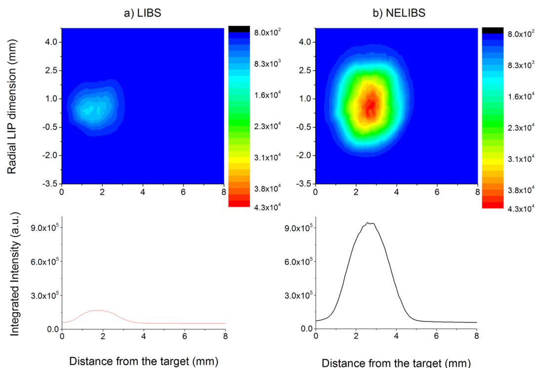
Figure 4. Total emission images of LIBS and NELIBS plasma of 1 \mu\text{L} of 1 ppm \text{PbCl}_2 (delay time from the laser pulse, 1.3 \mu\text{s} ; gate width, 500 ns; laser fluence, 16.3 \text{J cm}^{-2} ). In the case of NELIBS, 1 \mu\text{L} of Au-NPs solution 0.04 \text{mg mL}^{-1} was used.
