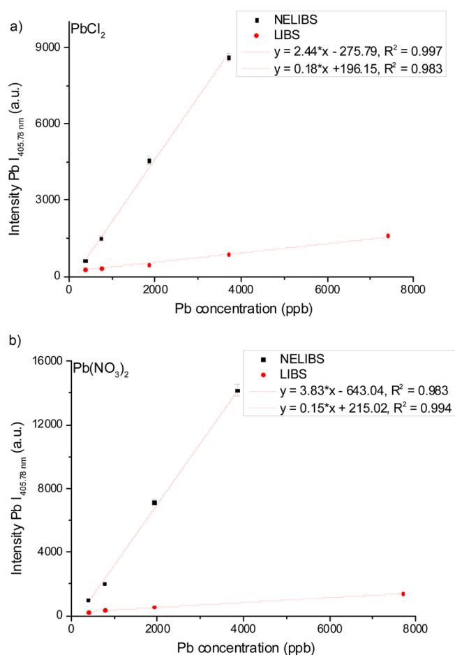
Figure 6. Calibration curve of Pb in the range of 0.5–8 ppm in the case of (a) \text{PbCl}_2 and (b) \text{Pb}(\text{NO}_3)_2 . Experimental conditions: 1 \mu\text{L} of sample solution; laser fluence, 16.3 \text{ J cm}^{-2} ; 1 \mu\text{L} of Au-NPs 0.04 \text{ mg mL}^{-1} .
