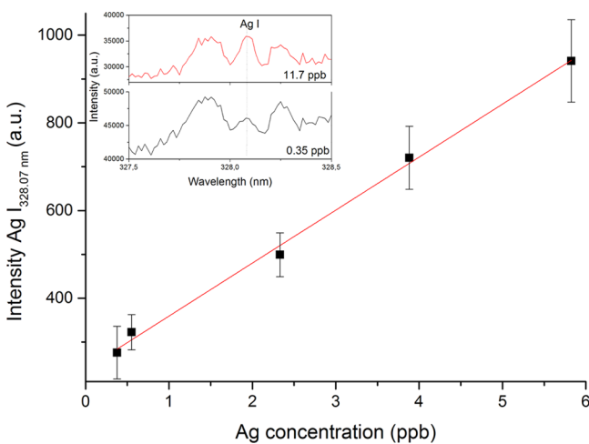
Figure 9. Calibration curve of Ag in the concentration range between 0 and 6 ppb. In the inset, the spectral line of Ag I at 328.07 nm at Ag concentrations of 11.7 and 0.35 ppb are shown. Experimental conditions: 1 \mu\text{L} of \text{AgNO}_3 sample solution; laser fluence, 12. \text{J cm}^{-2} ; 1 \mu\text{L} of Au-NPs (diameter of 20 nm) 0.03 \text{mg mL}^{-1} .
