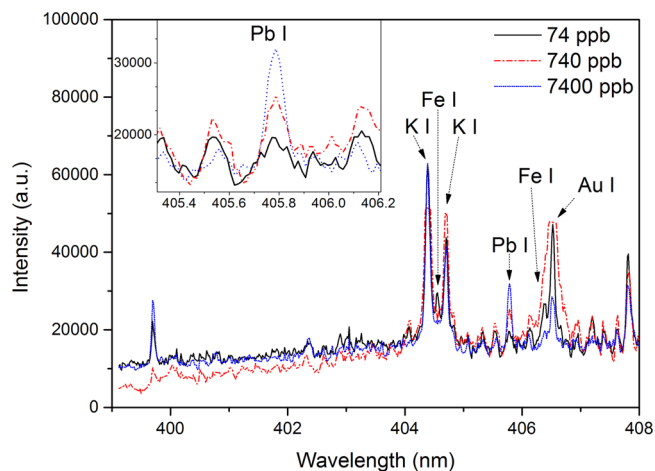
Figure 11. NELIBS spectra of human serum artificially contaminated with \text{PbCl}_2 at different concentrations: 74 ppb, 740 ppb, and 7400 ppb. The detector gain is different for each measurement in order to maximize the emission signal. Experimental conditions: laser fluence, 20.4 \text{J cm}^{-2} ; 1 \mu\text{L} of Au-NPs (diameter of 20 nm) 0.08 \text{mg mL}^{-1} .
