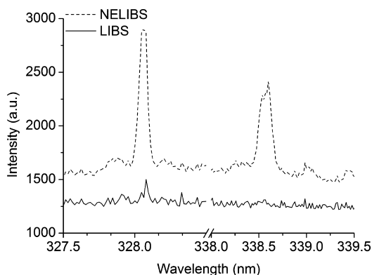
Figure 8. Comparison between the NELIBS and LIBS spectral line of Ag I (328.07 nm), for 1 \mu\text{L} of 100 ppb \text{AgNO}_3 solution. Experimental conditions: 1 \mu\text{L} of sample solution; laser fluence, 12. \text{J cm}^{-2} ; 1 \mu\text{L} of Au-NPs (diameter of 20 nm) 0.03 \text{mg mL}^{-1} .
