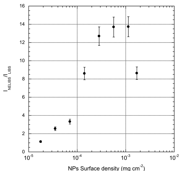
Figure 2. NELIBS spectral line enhancement of Pb I at 405.7 nm as a function of surface density of Au-NPs (diameter of 10 nm). The sample solution was 1 \mu L of 1 ppm PbCl 2 , laser fluence 16.3 J cm -2 .
