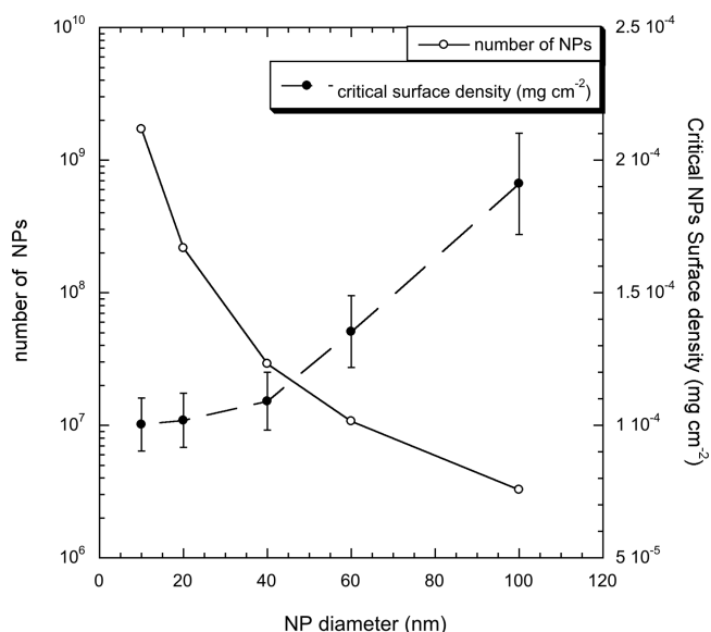
Figure 3. Critical surface density and corresponding number of NPs deposited on substrate surface as functions of NP diameter in NELIBS experiment.
