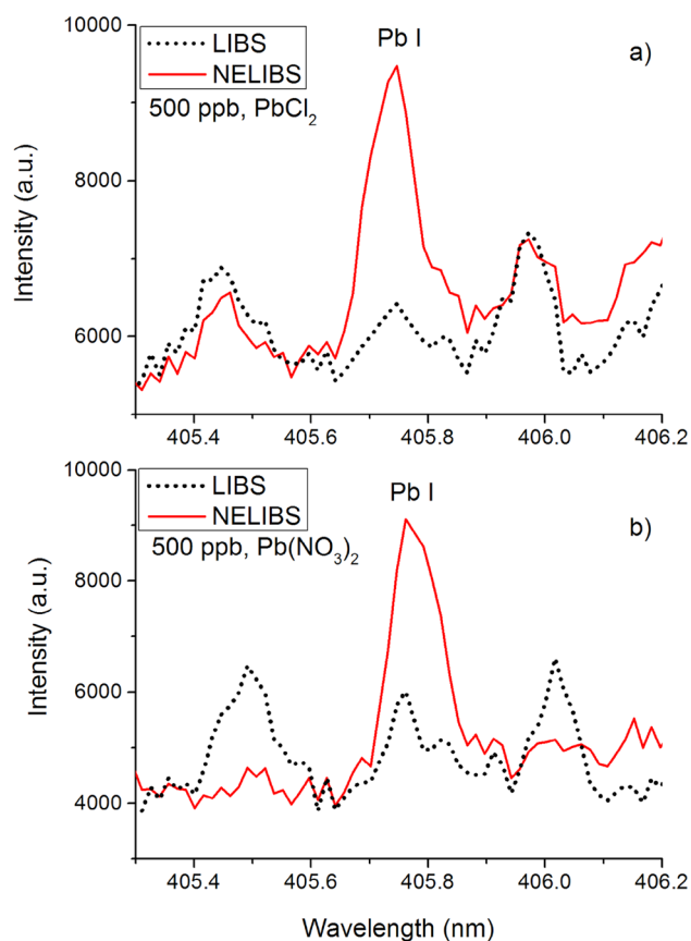
Figure 5. Comparison between the NELIBS and LIBS spectral line of Pb I (405.7 nm) for 1 \mu\text{L} of 500 ppb (a) \text{PbCl}_2 and (b) \text{Pb}(\text{NO}_3)_2 solutions. Experimental conditions: laser fluence, 16.3 \text{ J cm}^{-2} ; 1 \mu\text{L} of 0.04 \text{ mg mL}^{-1} Au-NPs.
