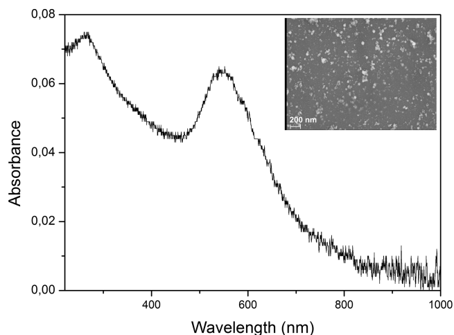
Figure 1. Absorption spectrum and SEM image of a glass substrate after the deposition of 1 \mu\text{L} of 2 \times 10^{-2} mg mL -1 Au-NPs before the NELIBS measurement.
